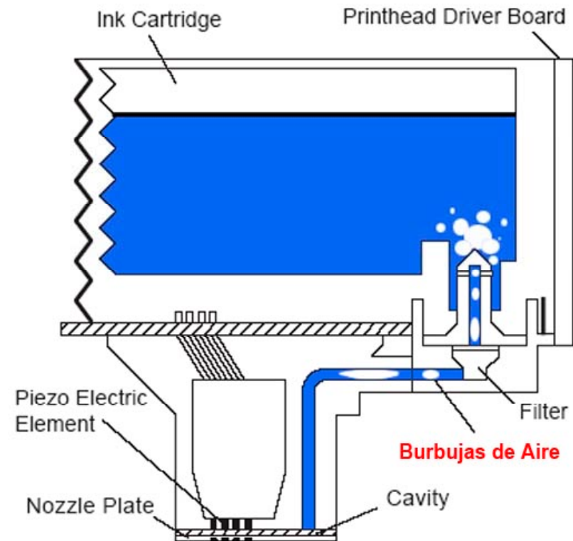
Figure 22. Printhead structure
